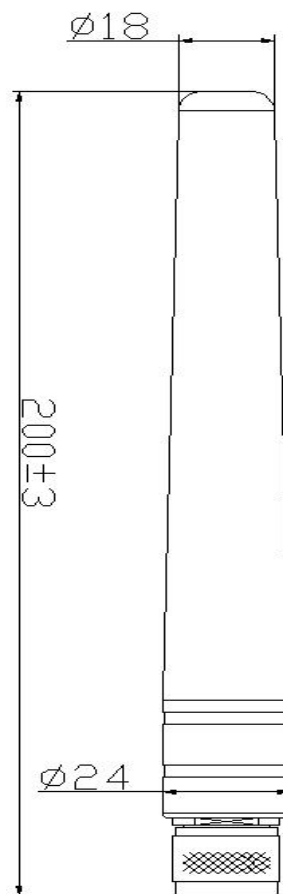
Installation Sketch
